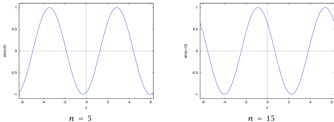
Figura 2.5 \sin(x + n)
