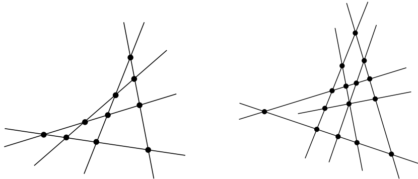
Figure 1: Two examples of sets satisfying GC_3 and GC_4 respectively.
