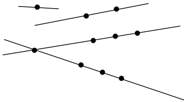
Figure 2: An example of a set satisfying (1.3)
