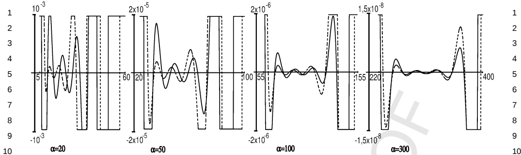
Fig. 2. Continuous lines represent the Charlier polynomial for n = 10 and several values of \alpha . Dashed lines represent the first term in the right-hand side of the expansion given in (5).
