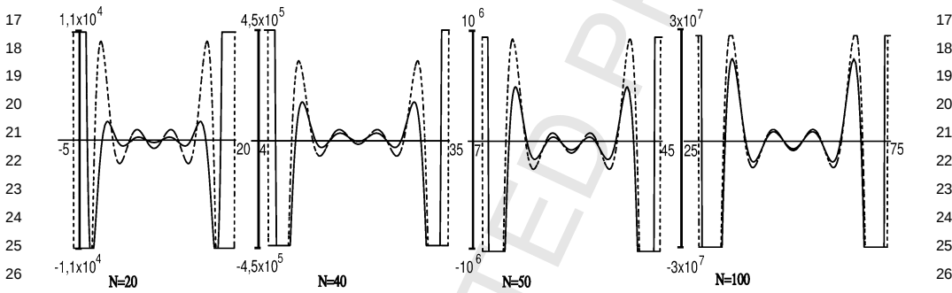
Fig. 3. Continuous lines represent the Krawtchouk polynomial for n = 10 , p = 1/2 , and several values of N . Dashed lines represent the first term in the right-hand side of the expansion given in (7).
