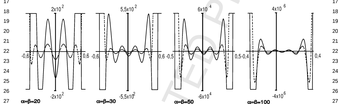
Fig. 6. Continuous lines represent the Jacobi polynomial for n = 10 and several values of \alpha = \beta . Dashed lines represent the first term in the right-hand side of the expansion given in (14)–(15).
