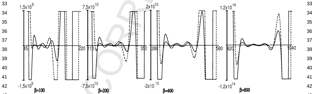
Fig. 4. Continuous lines represent the Meixner polynomial for n = 10 , c = 1/2 , and several values of \beta . Dashed lines represent the first term in the right-hand side of the expansion given in (9).
