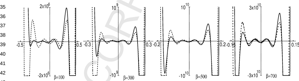
Fig. 10. Continuous lines represent the Jacobi polynomial for n = 10 and several values of \alpha = \beta . Dashed lines represent the first term in the right-hand side of the expansion given in (31)–(32).
