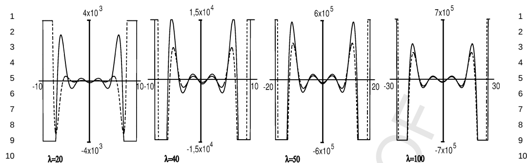
Fig. 5. Continuous lines represent the Meixner-Pollaczek polynomial for n = 10 , \phi = \pi/2 , and several values of \lambda . Dashed lines represent the first term in the right-hand side of the expansion given in (11)–(12).
