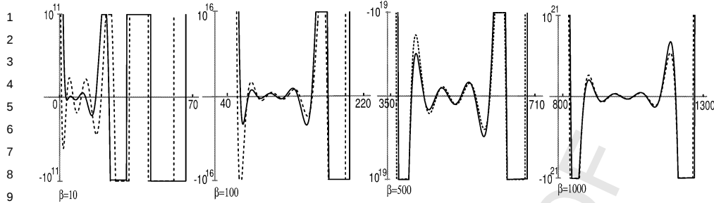
Fig. 8. Continuous lines represent the Meixner polynomial for n = 10 , c = 1/2 , and several values of \beta . Dashed lines represent the first term in the right-hand side of the expansion given in (25)–(26).
