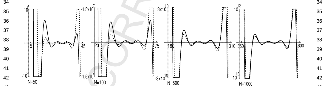
Fig. 7. Continuous lines represent the Krawtchouk polynomial for n = 10 , p = 1/2 , and several values of N . Dashed lines represent the first term in the right-hand side of the expansion given in (22)–(23).
