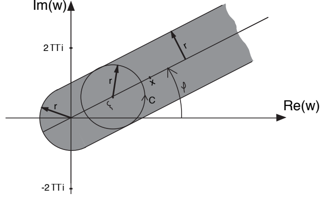
Figure 1. The circle of radius r \equiv \pi \cos \varphi centered at \xi , with \xi \in (0, x) , used in the Cauchy definition of r_{2N+2}(x) must be contained in the shaded region. This region is defined by the set \{w \in \mathcal{C}, |w - x| < \pi \cos \varphi, 0 \leq |x| < \infty\} .
