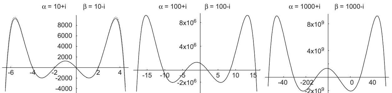
Fig. 8. Expansion (46). -(2a + 2b - 1)_6 p_6(x; \alpha, \beta, \bar{\alpha}, \bar{\beta})/[(2a)_6(a + b + i(c - d))_6] versus (C)_6 K_6(X; A, C) .
