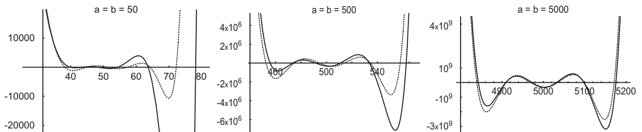
Fig. 2. Expansion (4) for c = 1 . S_6(x^2; a, b, 1)/[(a+b)_6 6!] versus P_6^{(C)}(X; A) .
