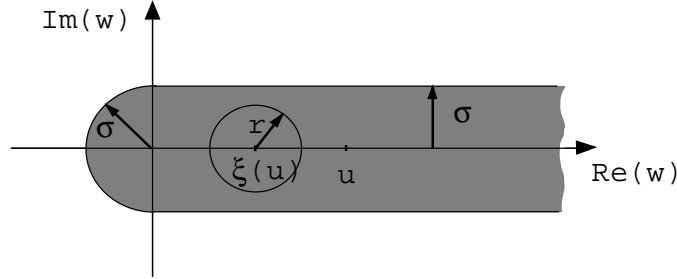
Figure 1: Analyticity region W for the function g(u) considered in lemma 5. The integration variable u in (9) is real and unbounded and therefore, the analyticity region for g(u) must contain the positive real axis. The circle of radius r centered at \xi(u) , with 0 < \xi(u) < u , used in the proof of lemma 5 must be contained in this region and therefore, r < \sigma .
