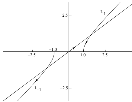
FIG. 3.2. Steepest descent path contour for F(z) of (3.5).
