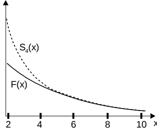
FIG. 2.1. Graphics of the approximation to the integral F(x) supplied by S_4(x) .
