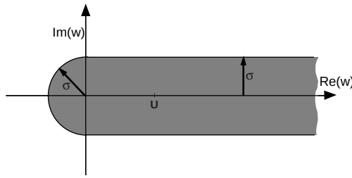
Figure 1. Analyticity region W for the function g(z) considered in proposition 3.
