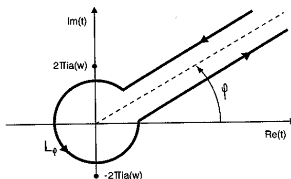
Fig. 1. Hankel's contour involved in the integral representation (3) of \zeta_2(v, z, w) . It surrounds the half-line [0, \infty e^{i\phi}) in the counterclockwise direction and does not enclose any pole \pm 2n\pi i , \pm 2n\pi i/w , n \in \mathbb{N} , of the integrand in (3). Then, in this picture, a(w) \equiv \text{Min}\{1, w^{-1}\} .
