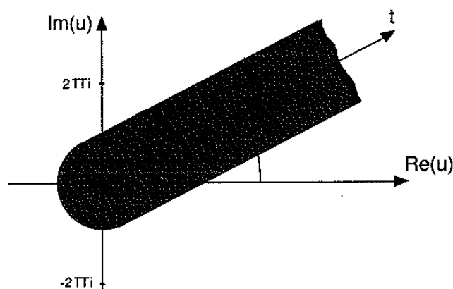
Fig. 2. The circle of radius r \equiv \pi \cos \varphi centered at \xi , with \xi \in (0, t) , used in the Cauchy definition of r_N(t) must be contained in the shaded region. This region is defined by the set \{u \in \mathbb{C}, |u - t| < \pi \cos \varphi, 0 \leq |t| < \infty, \text{Arg}(t) = \varphi\} .
